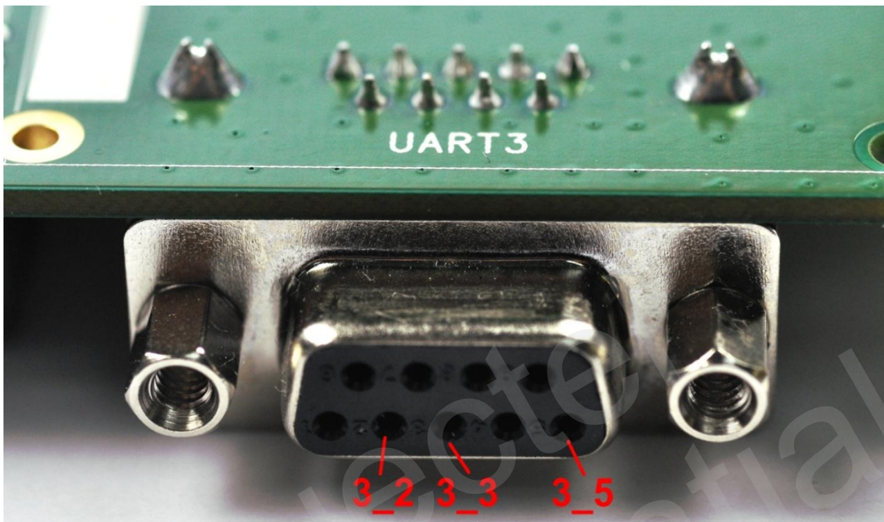
Figure 10: UART3
