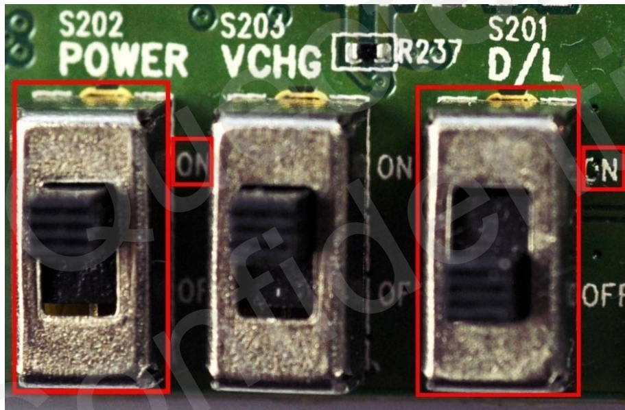
Figure 19: Switches State for Firmware Download
