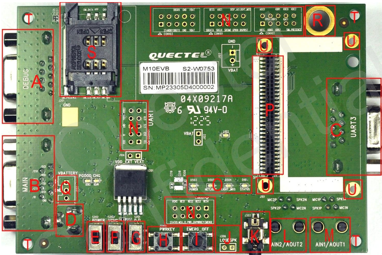
Figure 1: EVB Top View
