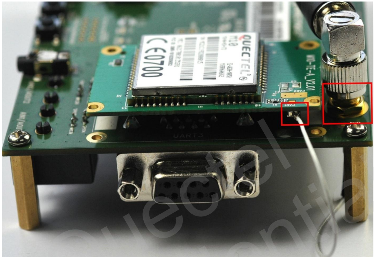
Figure 7: Antenna Interface
