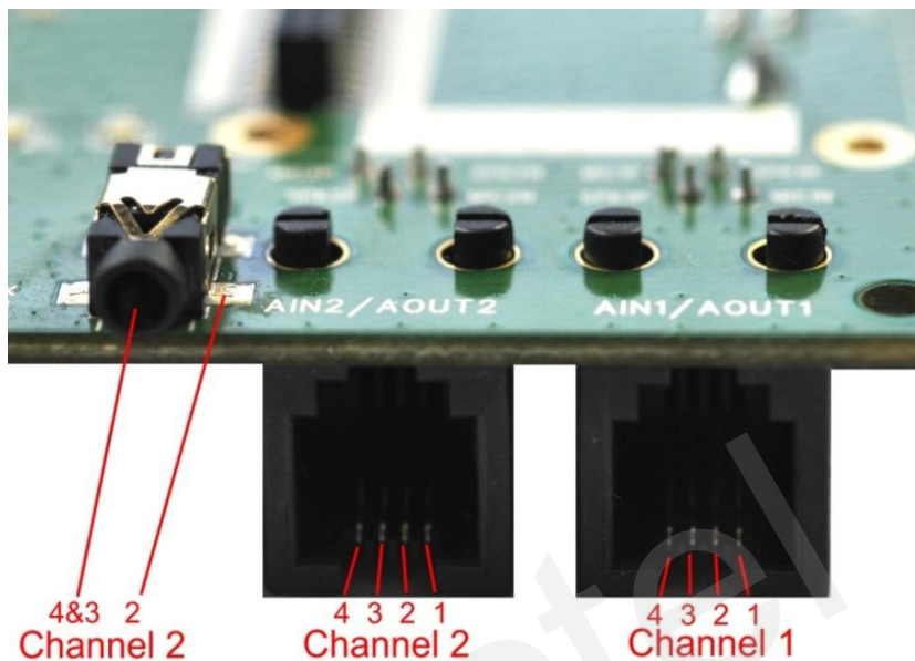
Figure 5: Audio Interface
