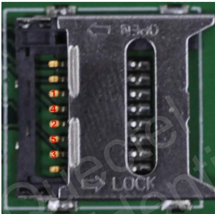
Figure 8: SD Interface
