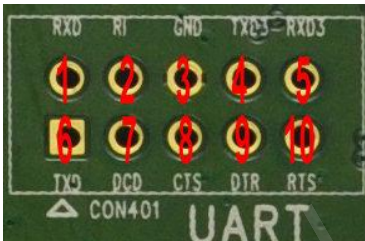
Figure 16: CON401 Points
